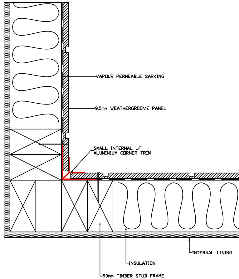
SMALL INTERNAL LF CORNER DETAIL
