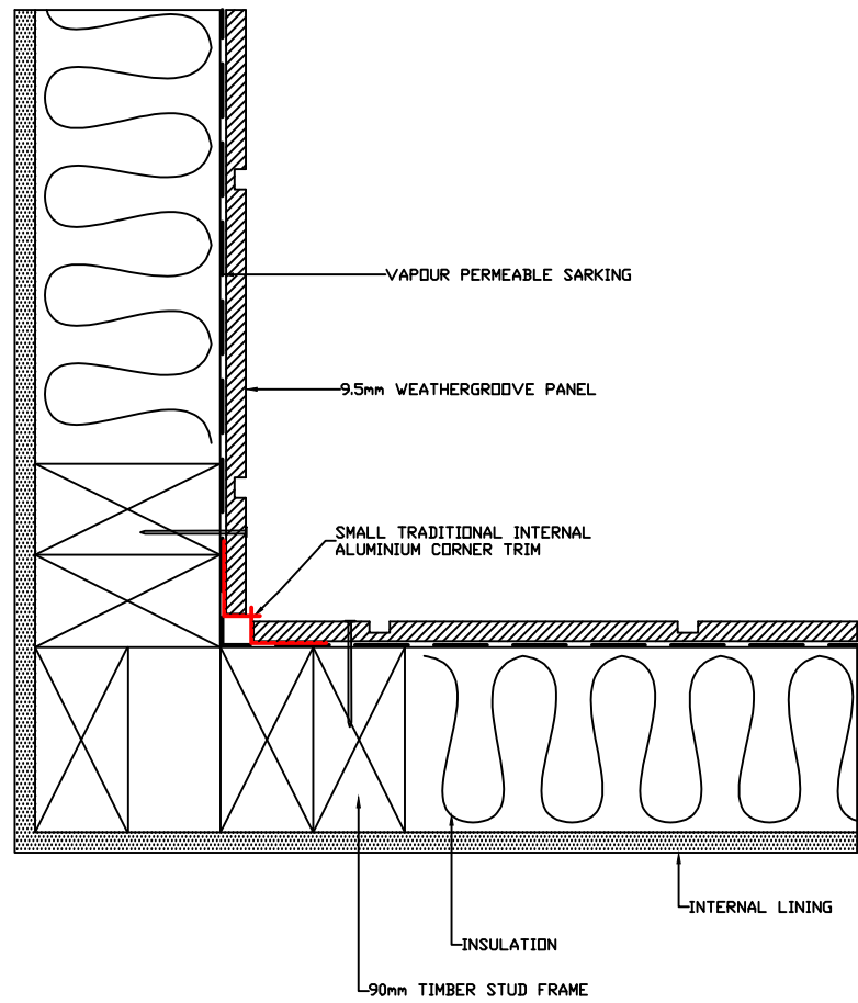
SMALL TRADITIONAL INTERNAL "W" CORNER DETAIL
