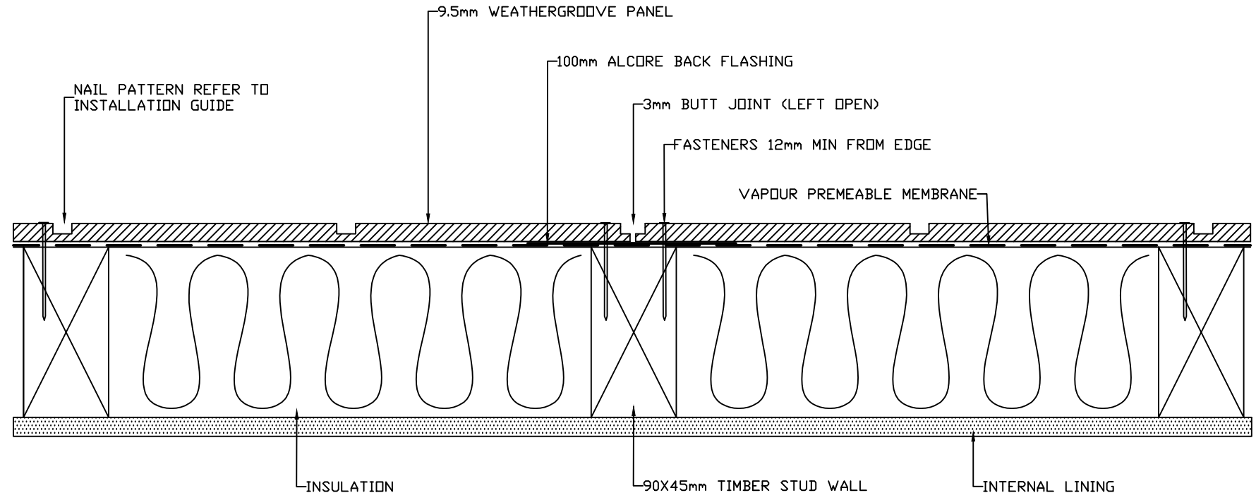
ON STUD BUTT JOIN DETAIL
