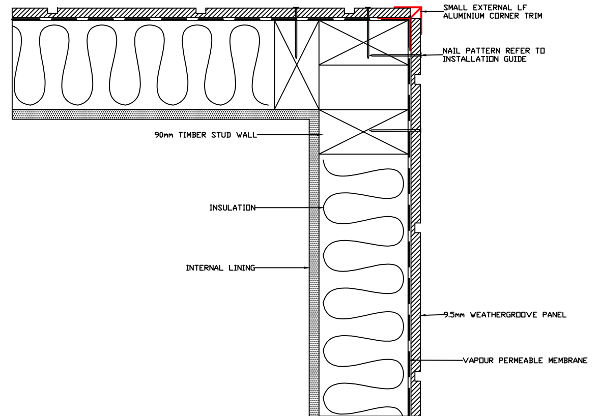
SMALL EXTERNAL LF CORNER DETAIL
