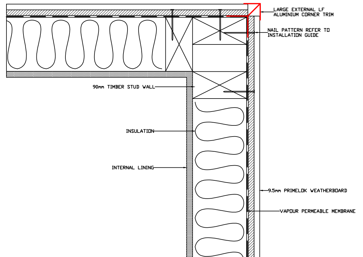
LARGE EXTERNAL LF CORNER DETAIL
