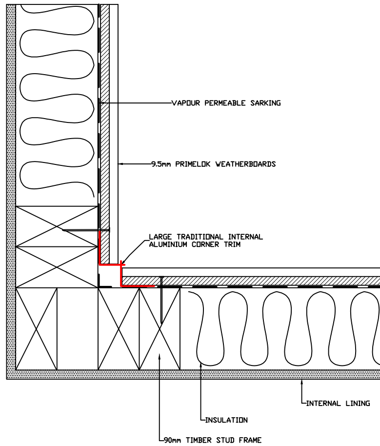
LARGE TRADITIONAL INTERNAL "W" CORNER DETAIL
