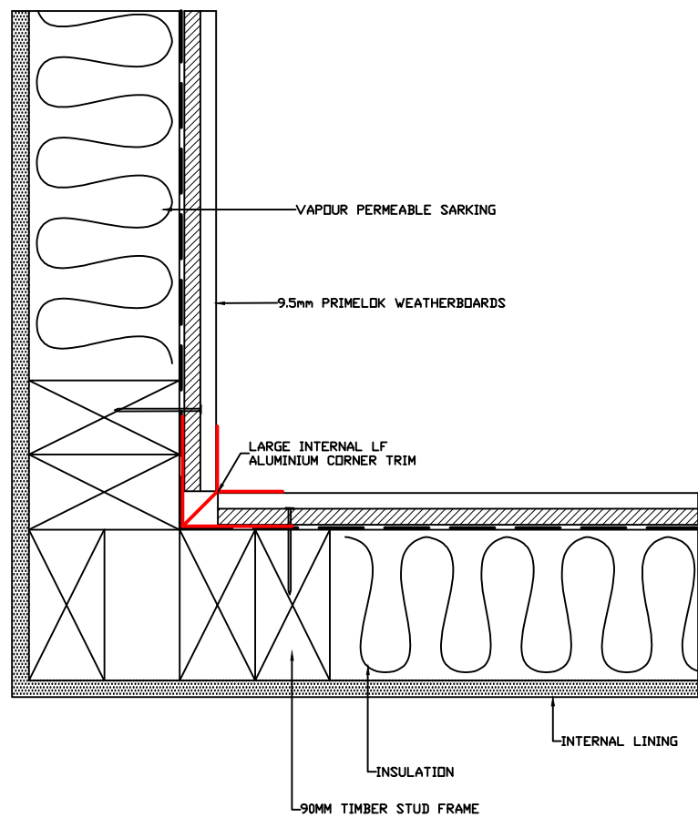
LARGE INTERNAL LF CORNER DETAIL
