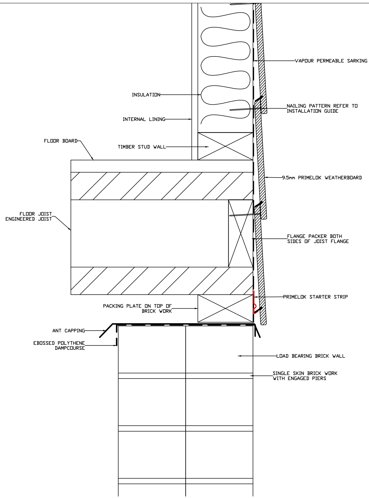
OVER DOUBLE BRICK PIER DETAIL
