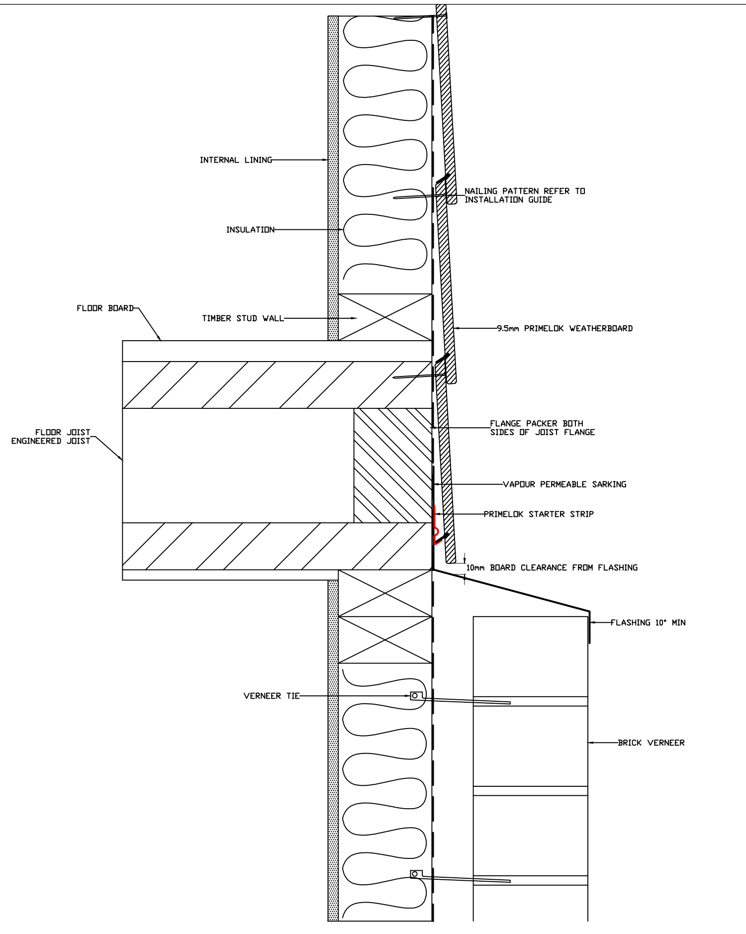
SET BACK OVER BRICK VENEER DETAIL
