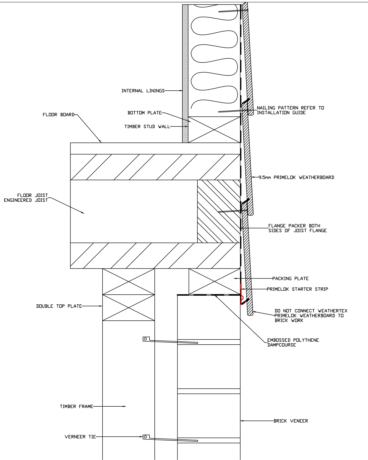
FLUSH WITH BRICK VENEER DETAIL
