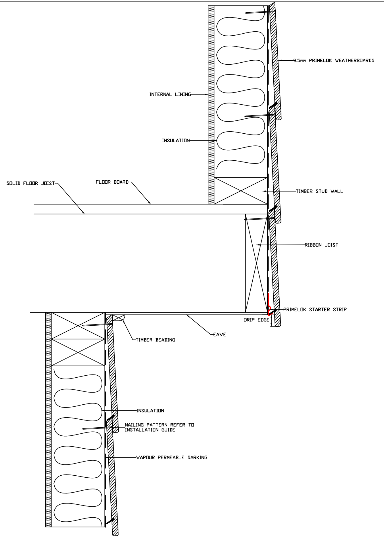
CANTILEVER ROOF DETAIL
