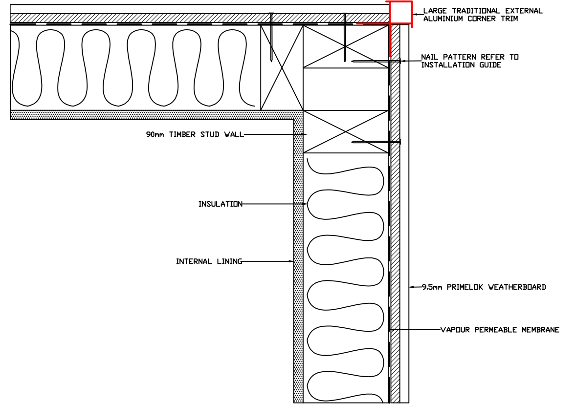
LARGE TRADITIONAL EXTERNAL "BOX" CORNER DETAIL
